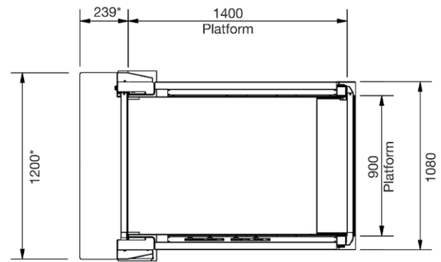
FOOTPRINT
