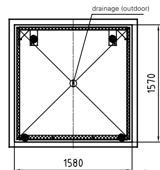
Basement view Max. slope 1% in the middle of the pit
